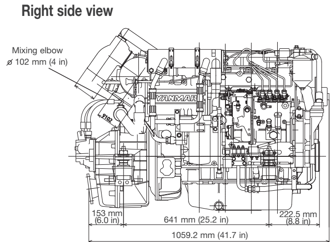
4LHA-DTP with ZF63A marine gear
