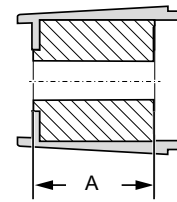
Long hub bushing A = 93mm (3.661")
