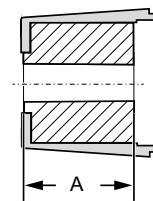
Short hub bushing A = 78mm (3.071")
