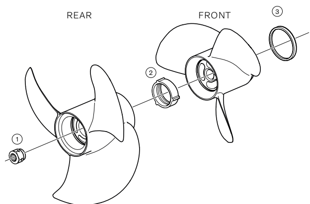
Type F, FH
